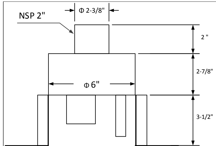
Side View, Units: Inches
